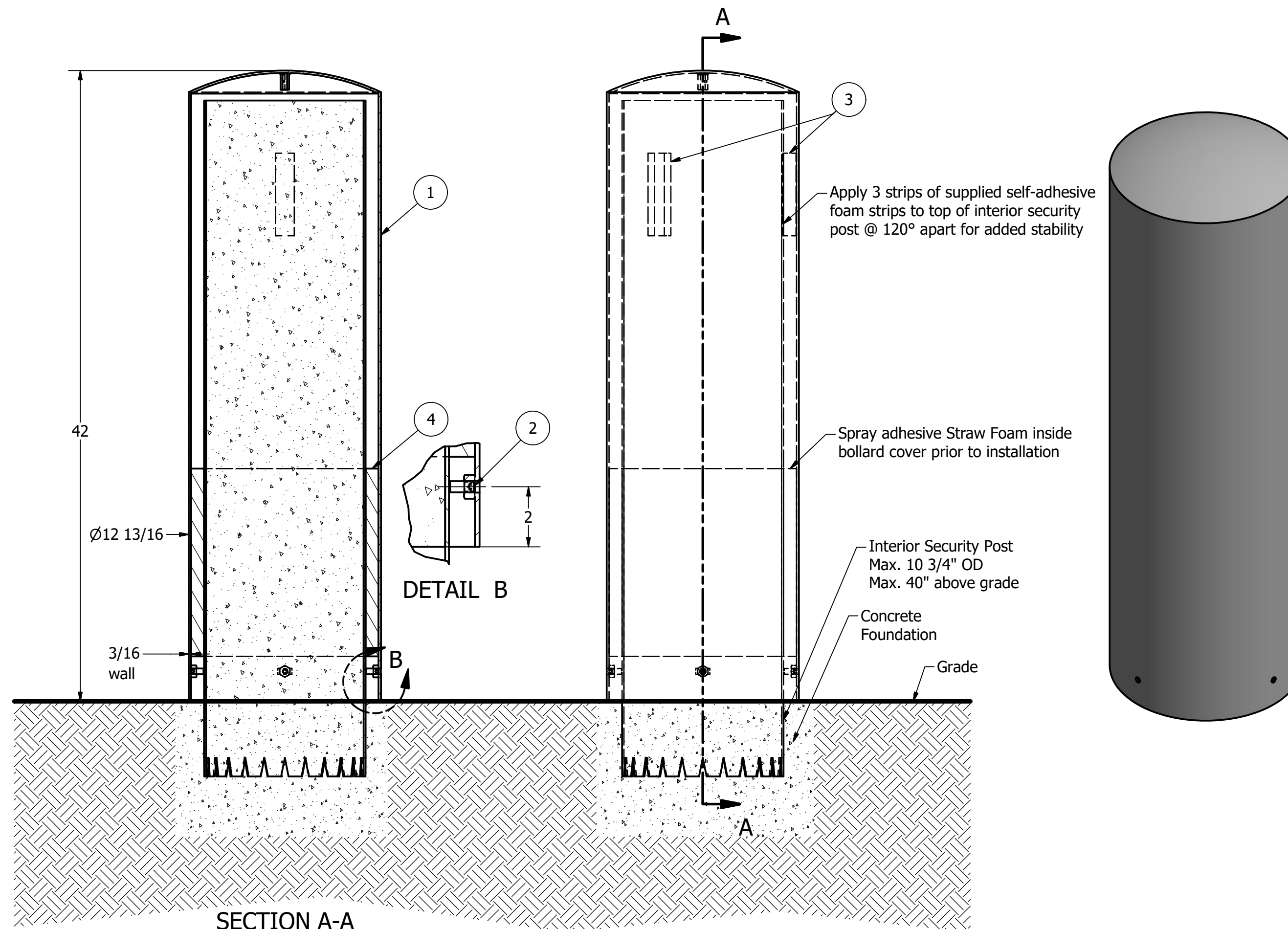
Adhesive Foam Installation Option
