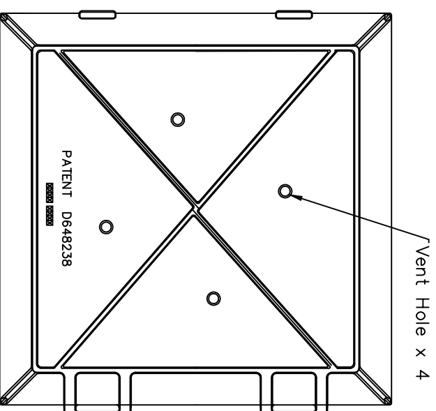
Underside View
