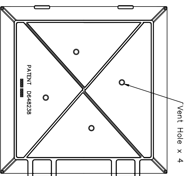
Underside View
