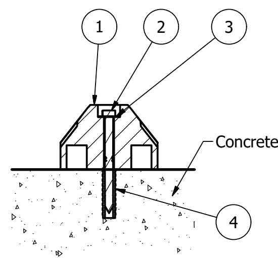
Concrete Installation w/ Lag Bolt and Lag Shield
